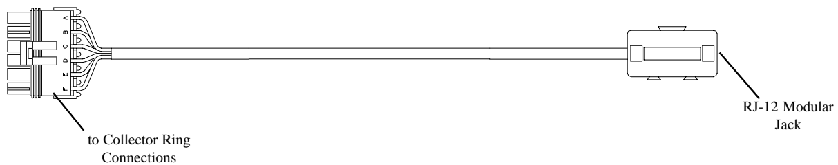
Figure 2: Turntable Interface Cable
