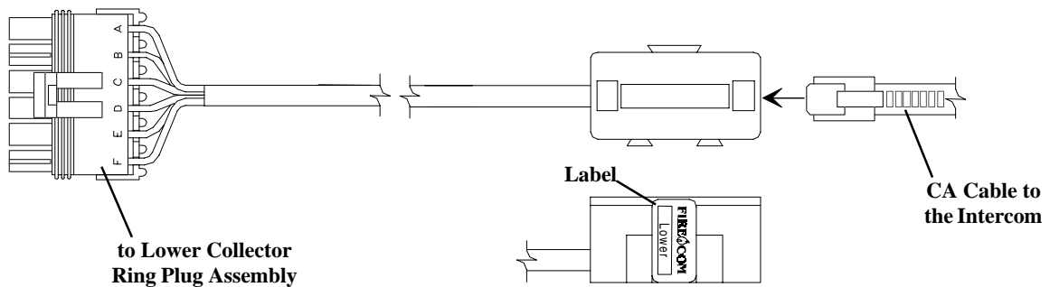
Figure 3: The Lower Interface Cable
