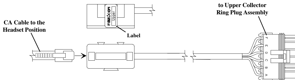
Figure 4: The Upper Interface Cable
